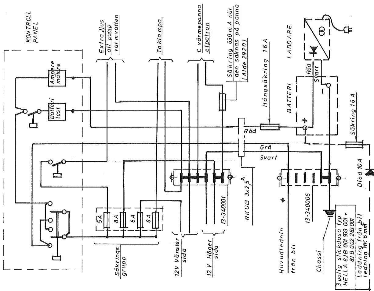
12 V system Caddy 84
